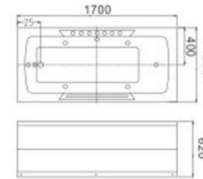
C-441 Size: 850x1500x620mm Size: 850x1600x620mm Size: 850x1700x620mm
