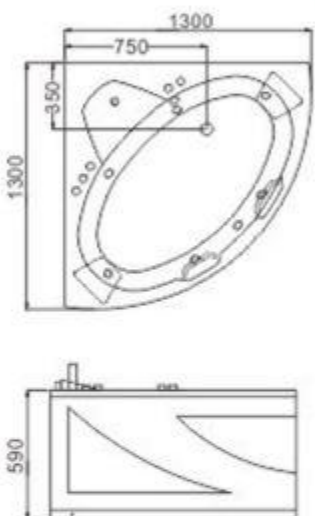
C-423 Size: 1300x1300x590mm
