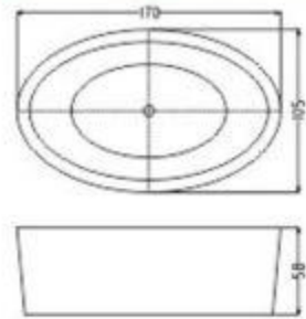
C-3154 Size: 1050x1700x580mm
