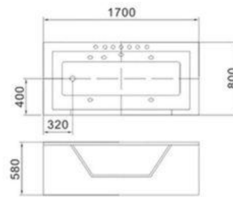
C-475 (R) Size: 800x1700x580mm
