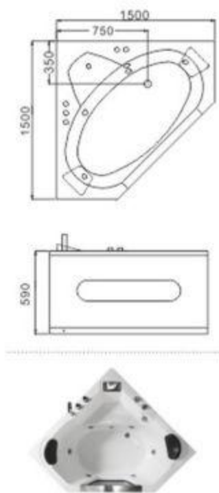
C-418 Size: 1500x1500x590mm
