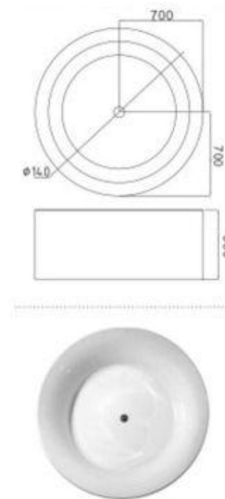
C-3173 Size: 1400x1400x580mm
