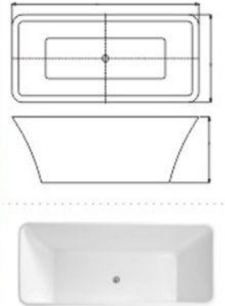
C-3147 Size: 700x1500x580mm Size: 750x1700x580mm
