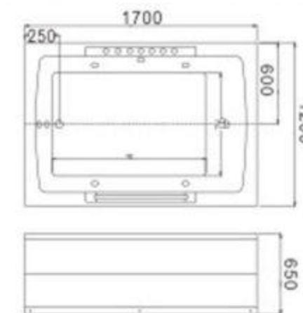
C-444 Size: 1200x1700x650mm
