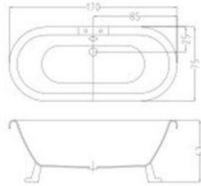
C-3166 Size: 750x1500x630mm Size: 750x1700x630mm
