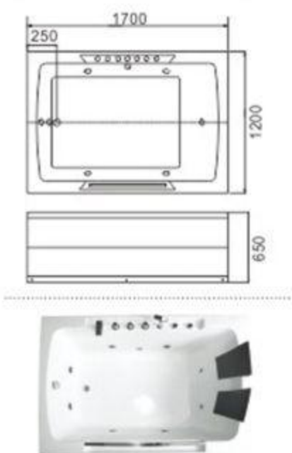
C-409 Size: 1200x1700x650mm
