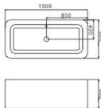
C-3008 Size: 800x1500x600mm
